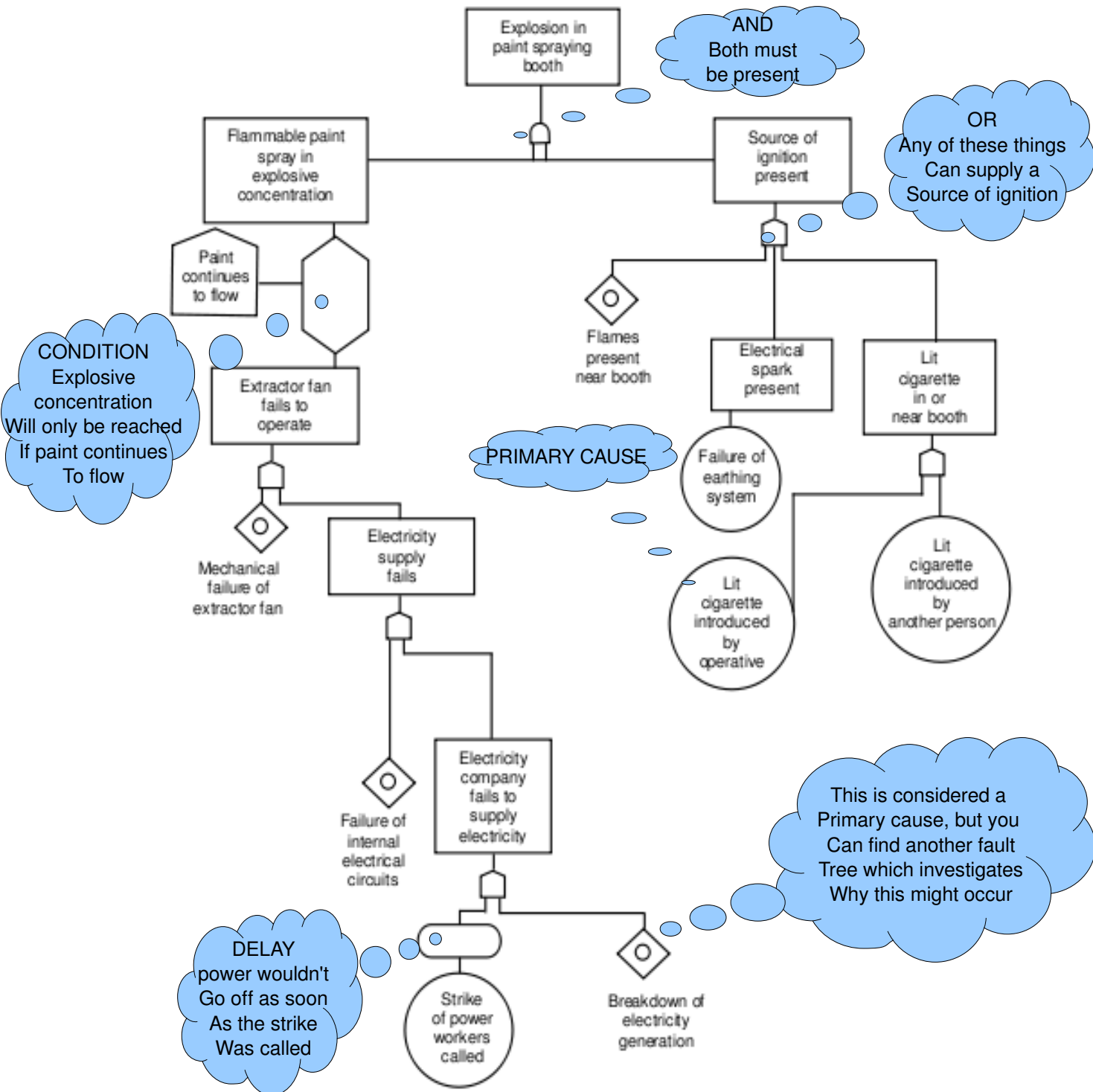
Simplified Fault Tree for the Top Event: "Explosion in Paint Spraying Booth"
